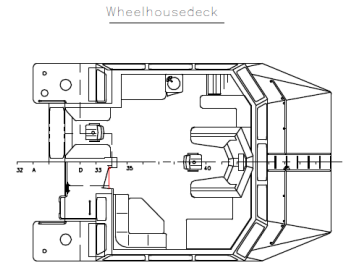
Wheelhouse deck
