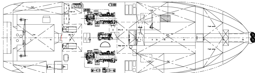
Below maindeck
