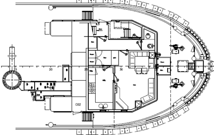
MAIN DECK/TANKTOP
