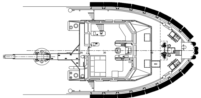
Forecastledeck
