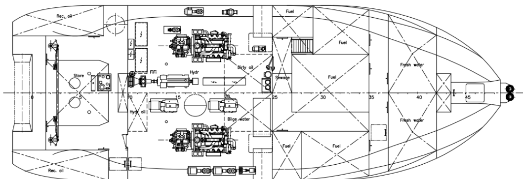
Below maindeck
