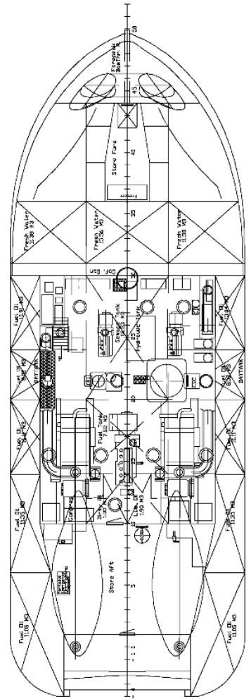
TANKTOP
