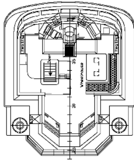
FORECASTLE DECK
