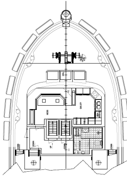
FORECASTLE DECK
