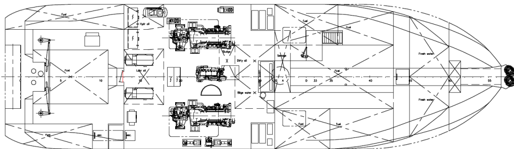
Below maindeck
