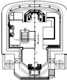
BRIDGE DECK
