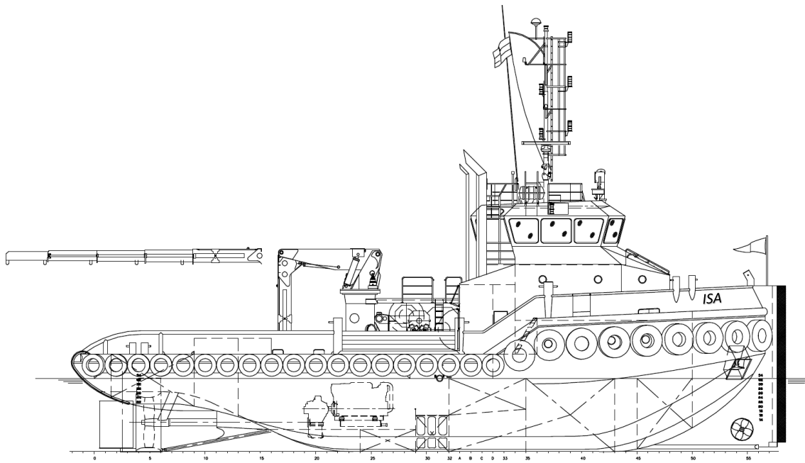
Forecastledeck
