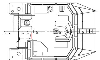
Wheelhousedeck
